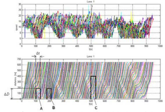
Figure 2. Upper/lower plot: individual vehicle speed /distance trajectories; distance trajectories were used for aggregation in a box with sides \Delta D and \Delta t to estimate traffic state parameters.
