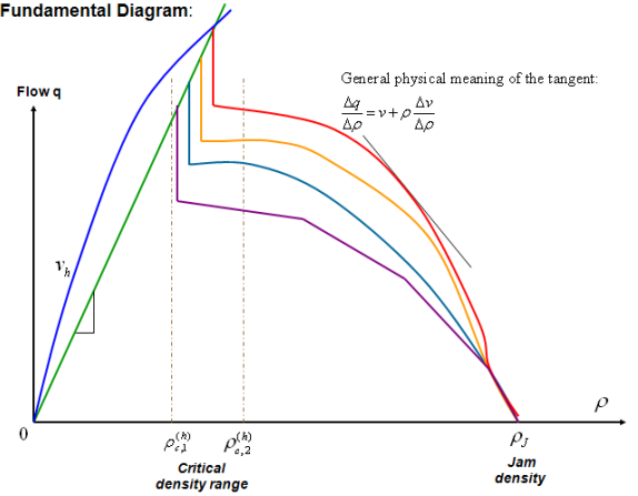
Figure 5. FD for homogenous flow; v_h is the speed of the homogenous flow; breakdown density for a homogenous flow falls into a range [\rho_{c,1}^h, \rho_{c,2}^h] which is different in time and locations.
